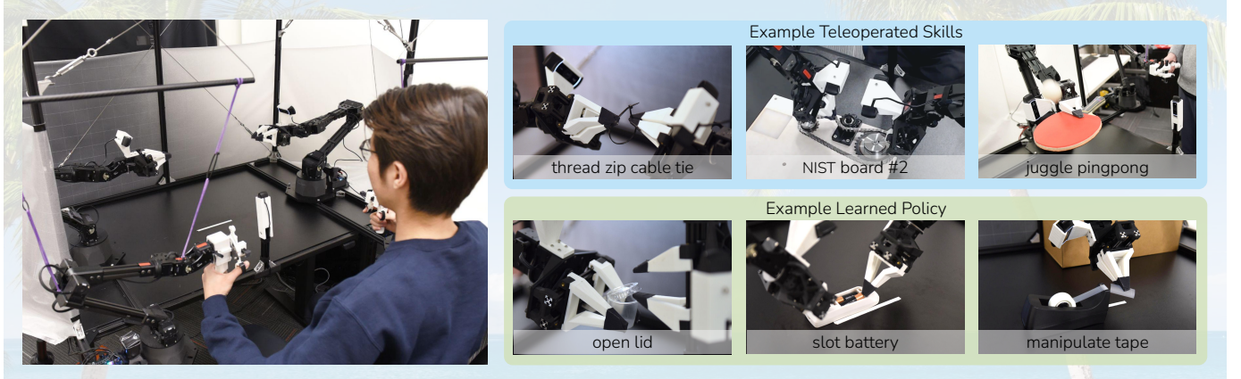
Fig. 1: ALOHA 🍷: A Low-cost Open-source Hardware System for Bimanual Teleoperation. The whole system costs <$20k with off-the-shelf robots and 3D printed components. Left : The user teleoperates by backdriving the leader robots, with the follower robots mirroring the motion. Right : ALOHA is capable of precise, contact-rich, and dynamic tasks. We show examples of both teleoperated and learned skills.
